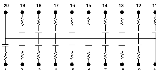
SCHEMATIC V
