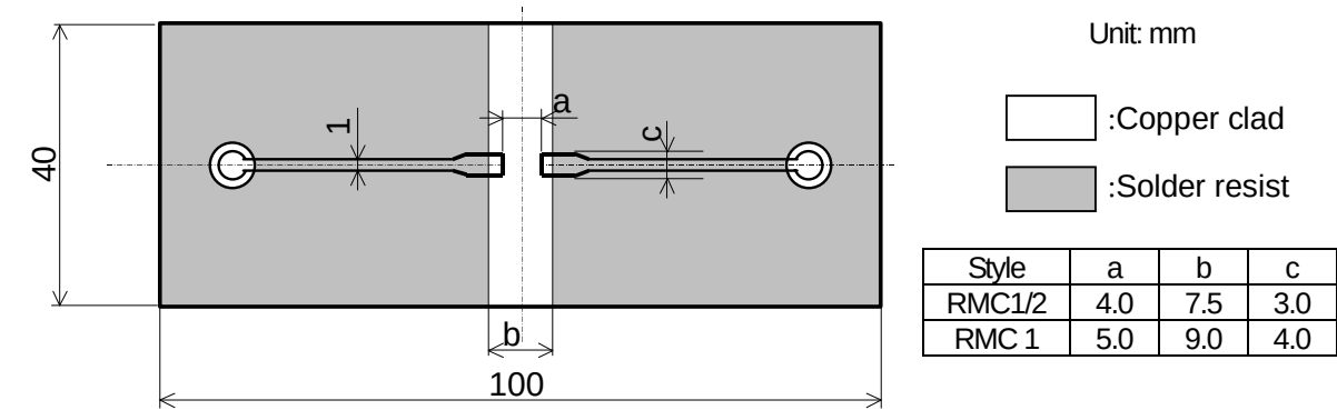
RMC1/2, 1 BOUND STRENGTH OF THE END FACE PLATING TEST SUBSTRATE
