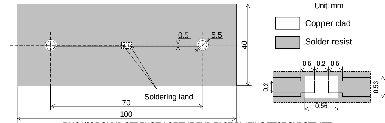
RMC1/32 BOUND STRENGTH OF THE END FACE PLATING TEST SUBSTRATE Thickness: 1.6mm Thickness of copper clad: 0.035mm Figure-4
