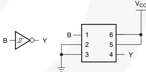
Figure 7. Inverter
