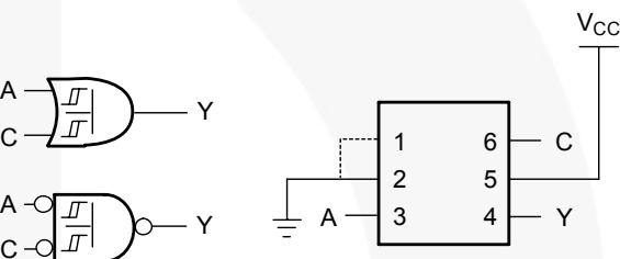
Figure 5. 2-Input OR Gate or 2-Input NAND Gate with Both Inputs Inverted
