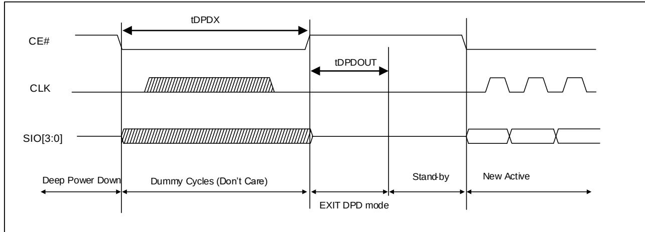
Figure 5.15 DEEP POWR DOWN EXIT Timing
