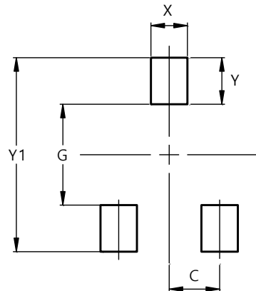
SOT323 (Standard)
