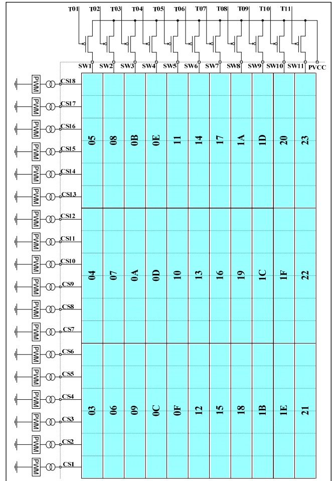
Figure 12 Open Register
