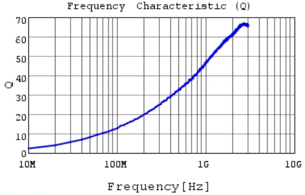
LQP03HQ3N6B02 Q
