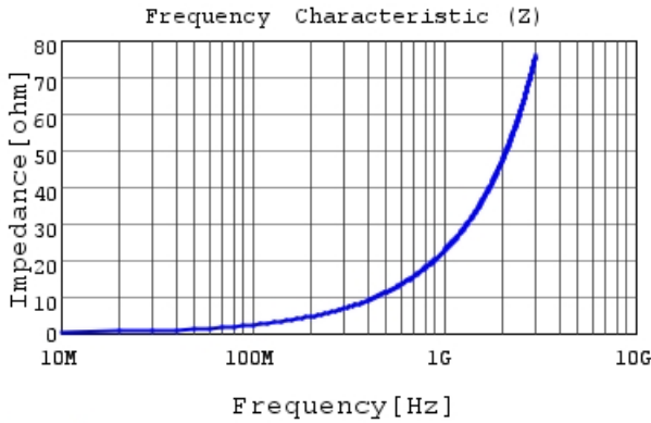
LQP03HQ3N6B02 |Z|
