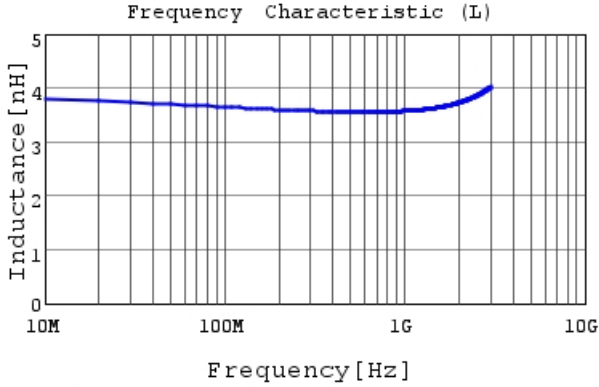
LQP03HQ3N6B02 L
