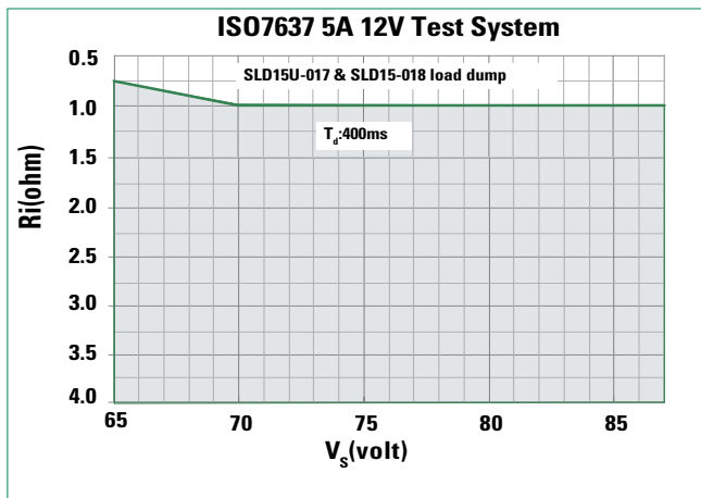
Figure 6 - SOA Chart
