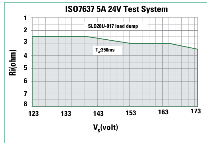
Figure 6 - SOA Chart
