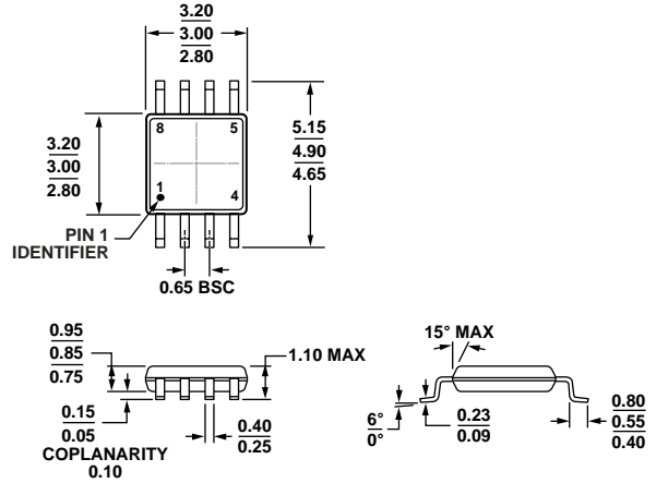
Figure 32. 8-Lead Mini Small Outline Package [MSOP] (RM-8)
