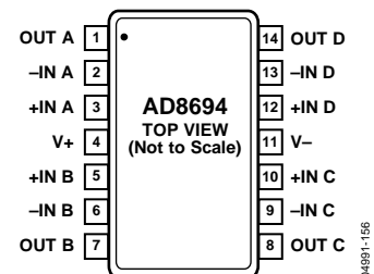
Figure 4. 14-Lead SOIC and 14-Lead TSSOP
