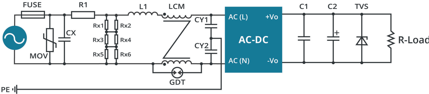
Figure 3 RECCOMENDED CIRCUIT FOR CLASS I EQUIPMENT
