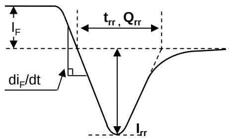
Fig.25 Diode Revere Recovery Waveform
