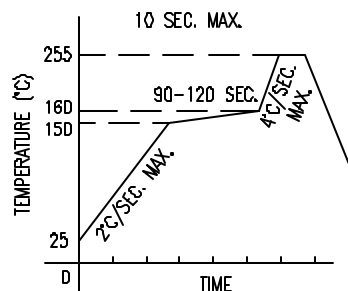
LEAD FREE REFLOW PROFILE
