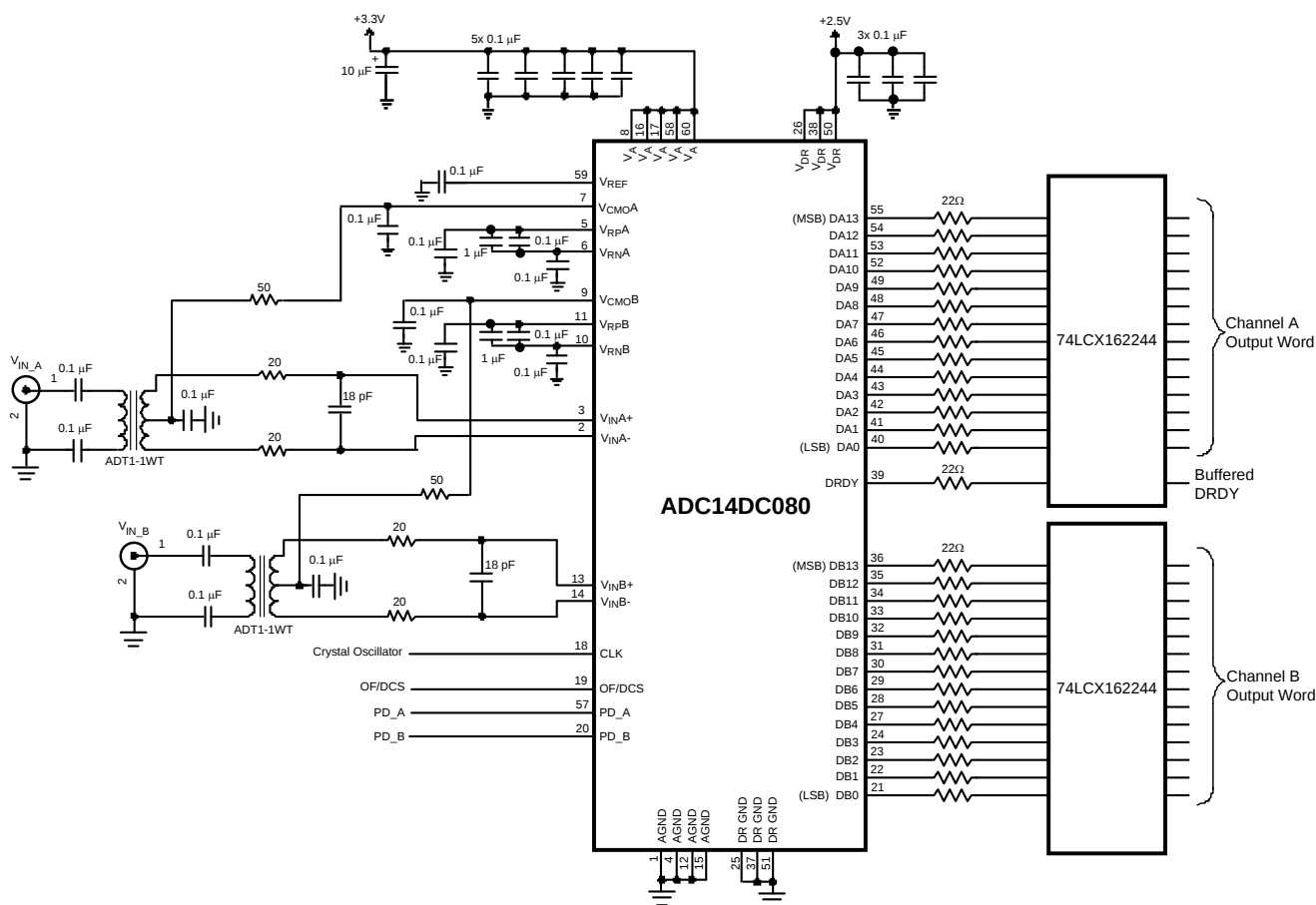
Figure 21. Application Circuit
