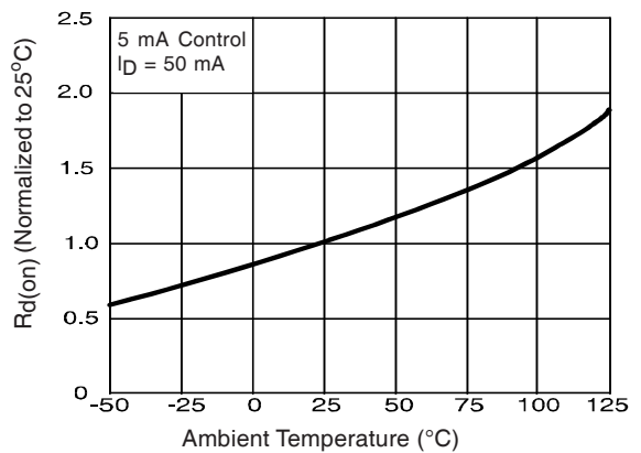
Figure 4. Typical On-Resistance
