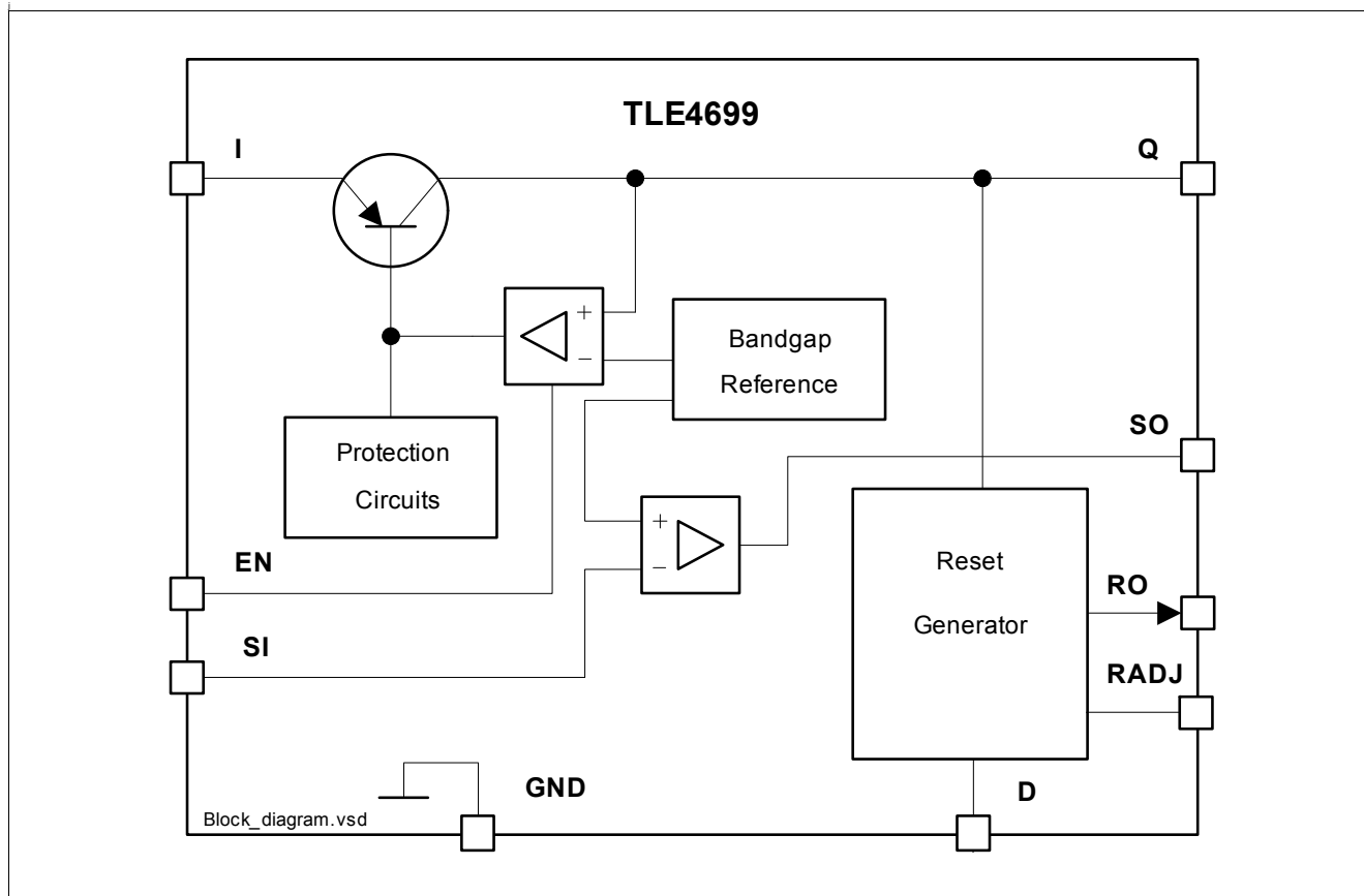
Figure 1 Block Diagram TLE4699
