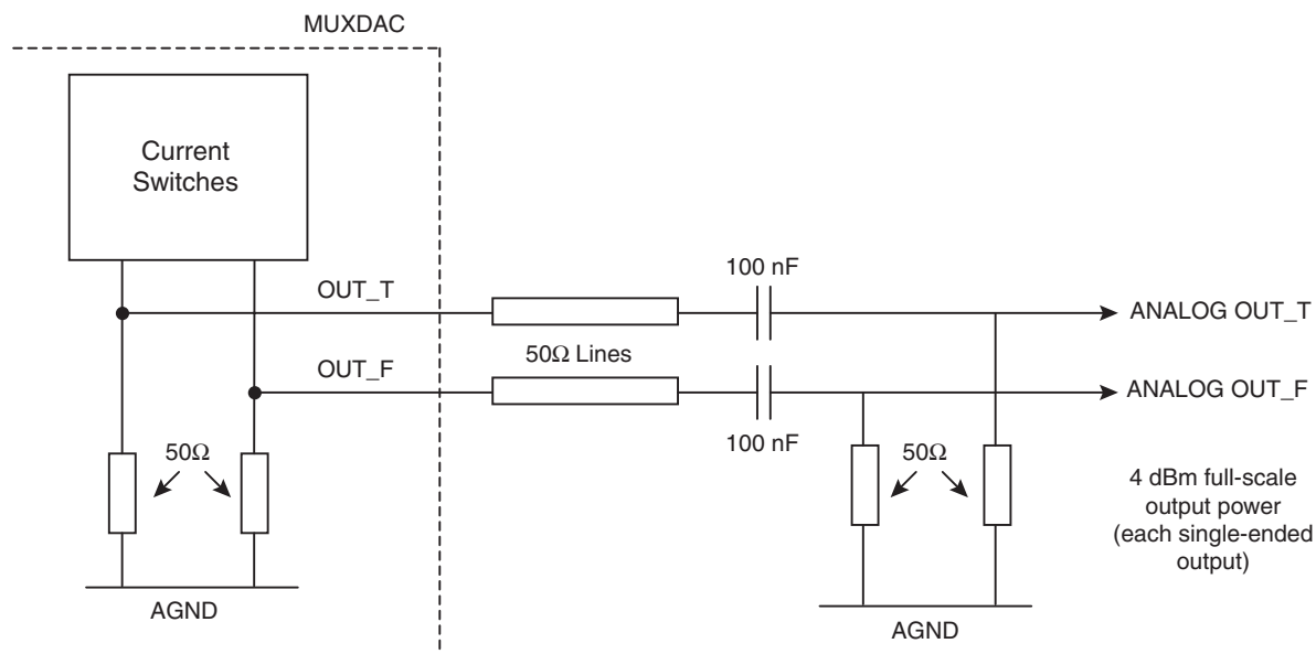
Figure 12-13. Analog Output 2 \times 50\Omega Differential Termination Scheme
