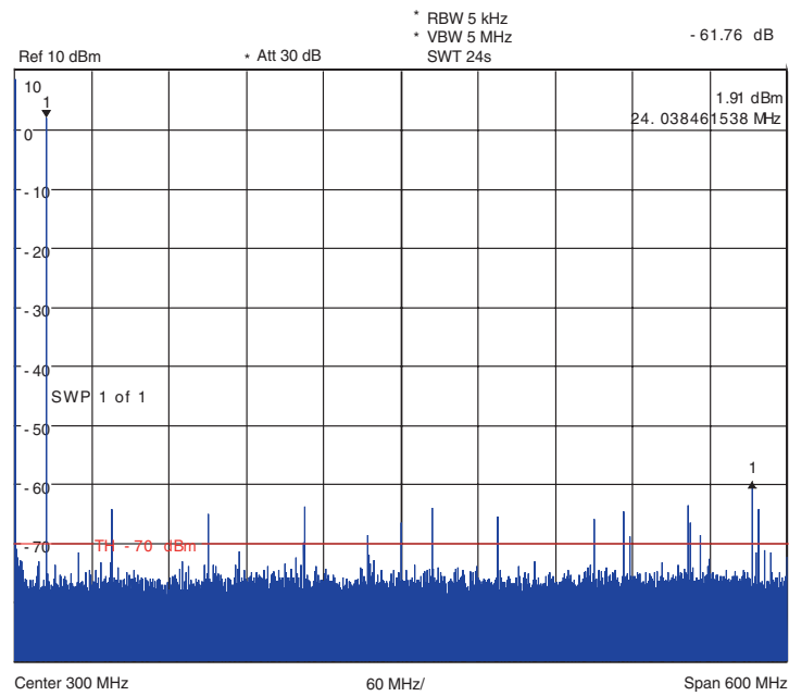
Figure 3-3. Single-tone Spectrum in First Nyquist F_s = 1.2 Gsps in First Nyquist Zone ( F_{out} = 25 MHz, -6 dBFS) SFDR = 62 dBc (68 dBFS)
