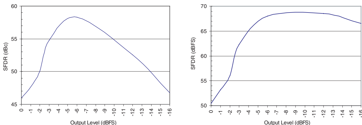
Figure 3-1. SFDR at F_s = 1.2\text{ Gsps} Against Output Level in Nyquist Conditions ( F_{out} = 575\text{ MHz} )
