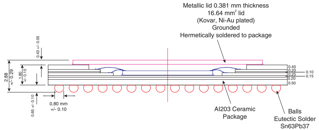
Figure 13-3. CBGA 255 Package Outline – Cross Section
