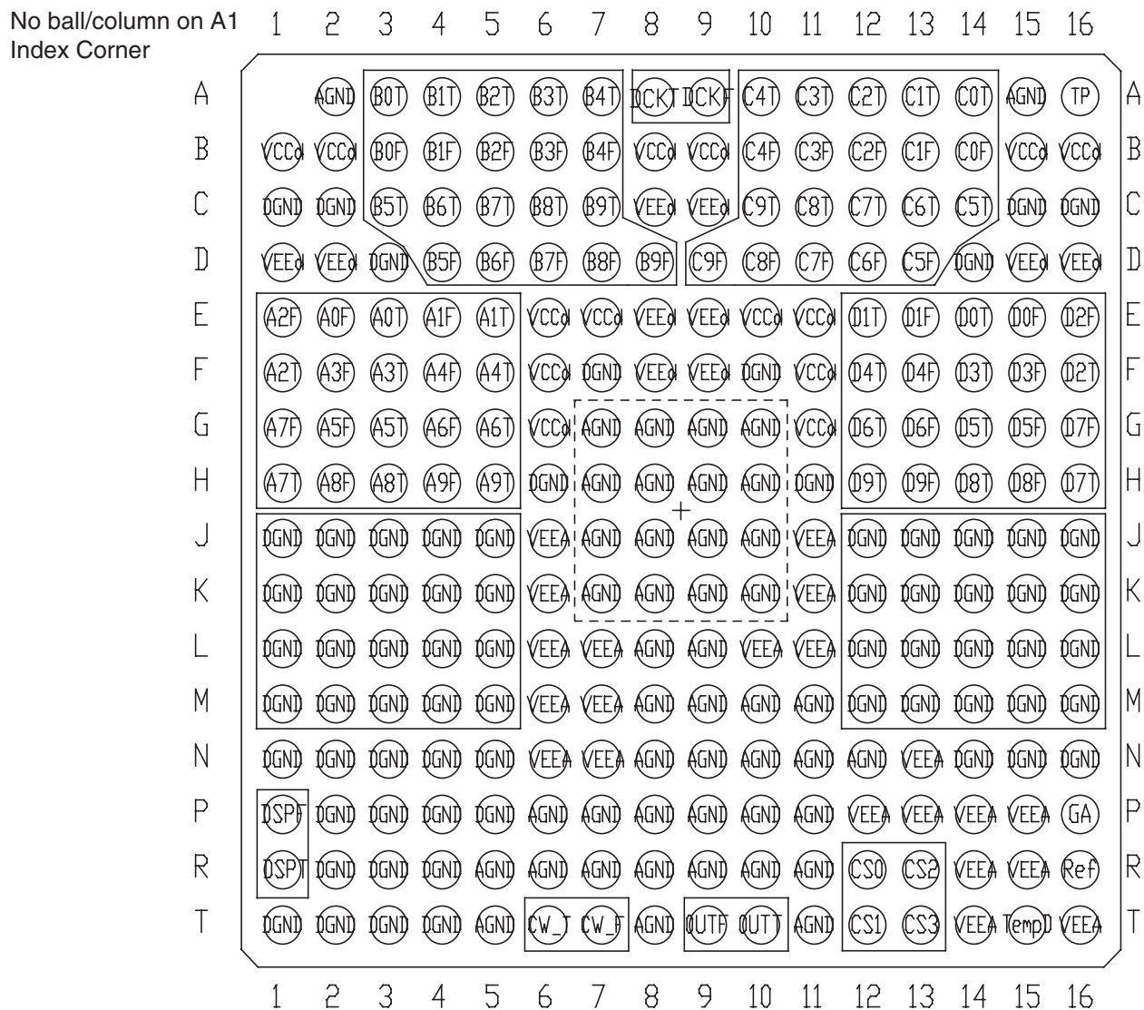
Figure 4-1. TS86101G2B Pin Configuration (Top View)
