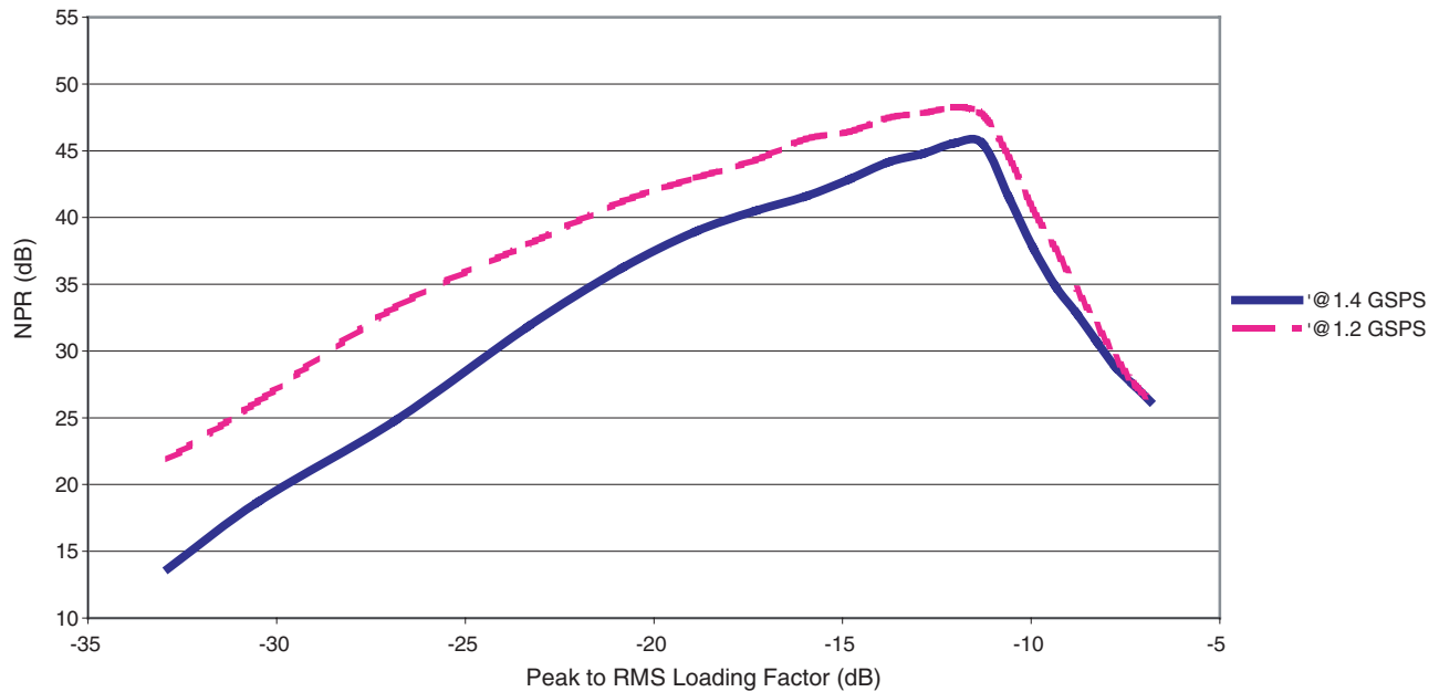
Figure 3-13. Noise Power Ratio (NPR) Against Peak to RMS Loading Factor F_s = 1.2 Gsps, 20 to 580 MHz Broadband Pattern, 25 MHz Notch Centered Around 250 MHz F_s = 1.4 Gsps, 20 to 680 MHz Broadband Pattern, 25 MHz Notch Centered Around 250 MHz
