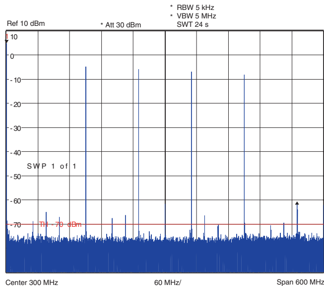
Figure 3-10. Four-tone Spectrum in First Nyquist Zone F_s = 1.2 Gsps 100 MHz spacing (-12 dBFS): F_{out1} = 150 MHz, F_{out2} = 250 MHz, F_{out3} = 350 MHz, F_{out4} = 450 MHz Four-tone IMD = 68 dBFS
