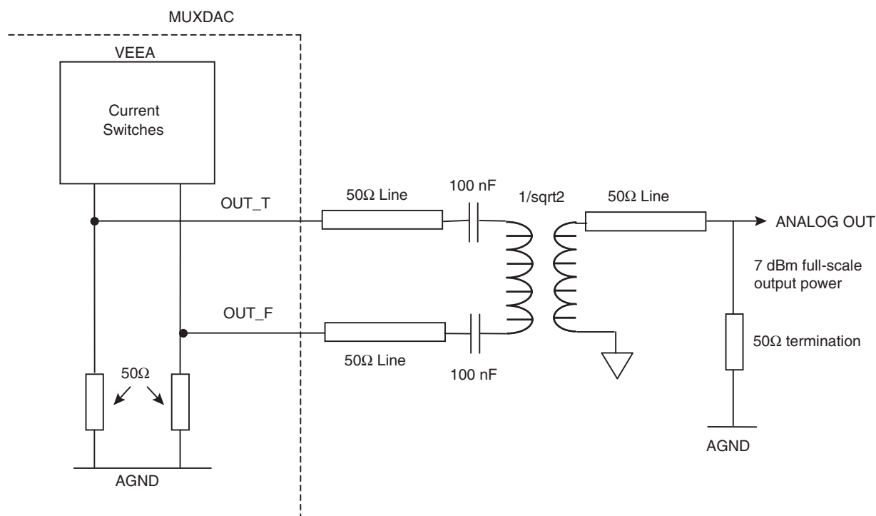
Figure 12-14. 50\Omega Single-ended Output through a Differential to Single-ended 1/\sqrt{2} Balun (1/ \sqrt{2} voltage ratio is necessary for correct 100\Omega differential to 50\Omega single-ended impedance transformation)
