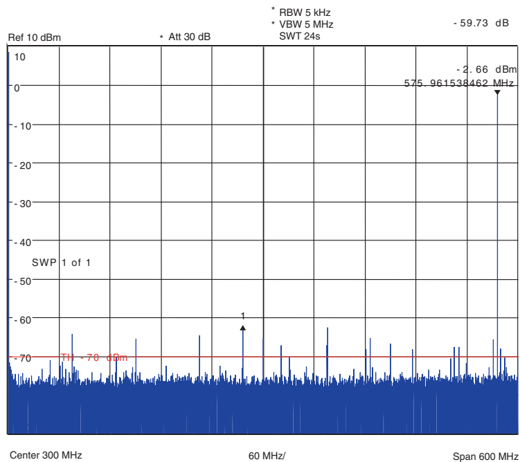
Figure 3-4. Single-tone Spectrum in First Nyquist F_s = 1.2 Gsps in First Nyquist Zone ( F_{out} = 575 MHz, -6 dBFS) SFDR = 59 dBc (69 dBFS)
