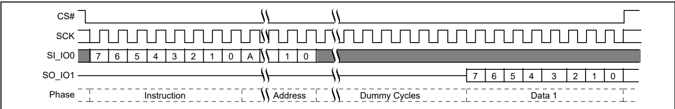
Figure 31 RSFDP command sequence
