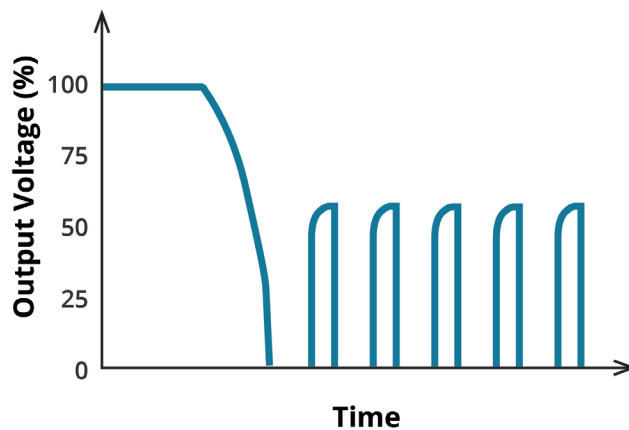
OUTPUT VOLTAGE VS TIME HICCUP MODE
