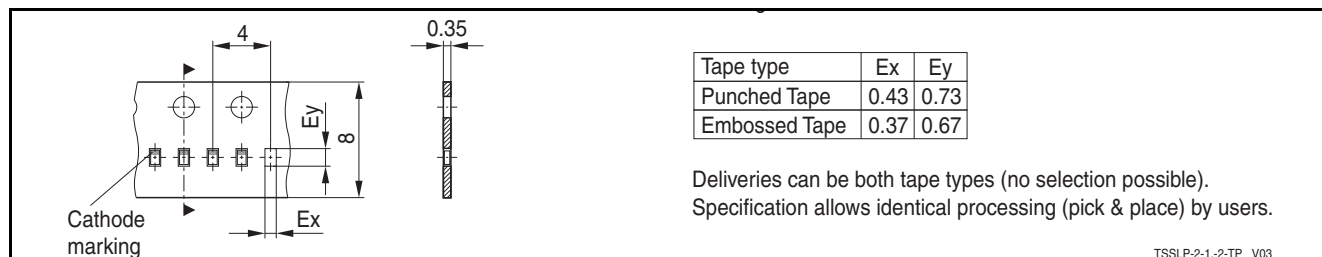
Figure 6-3 PG-TSSLP-2-1: Packing
