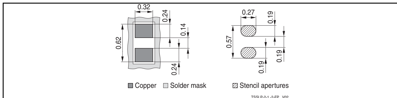
Figure 6-2 PG-TSSLP-2-1: Footprint
