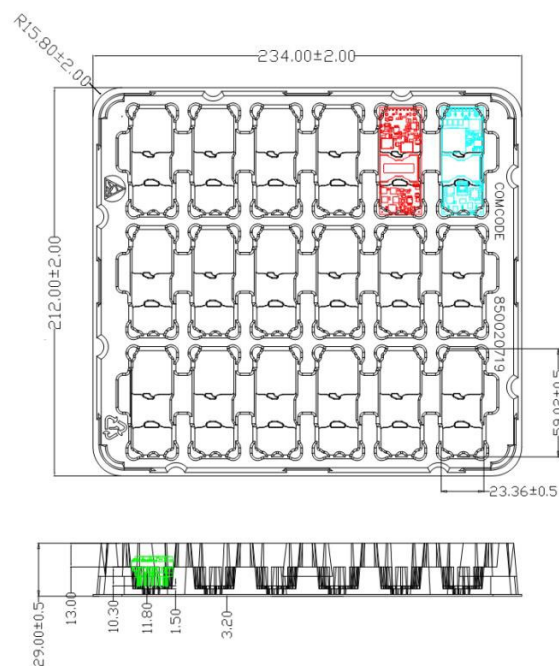
Base Plate Module Tray
