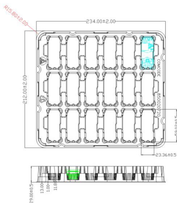
Open Frame Module Tray
