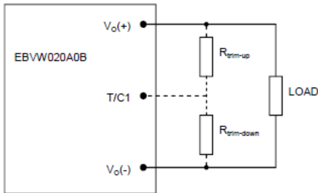
Figure 17. Circuit Configuration to Trim Output Voltage.
