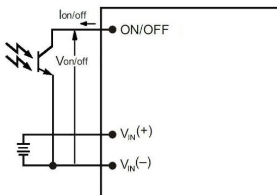
Figure 15. Remote On/Off Implementation.
