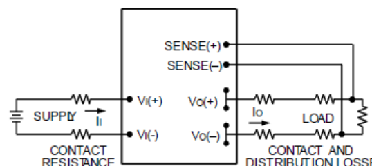
Figure 16. Circuit Configuration for remote sense.
