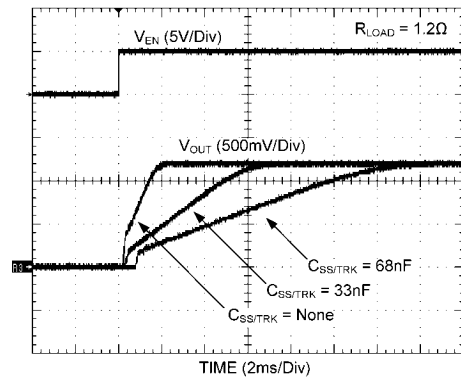
Start-Up (Soft-Start)
