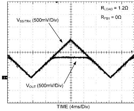
Start-Up (Tracking)
