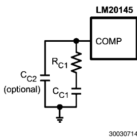
FIGURE 5. Compensation Network for LM20145
