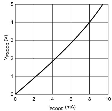
P_{GOOD} vs. I_{PGOOD}
