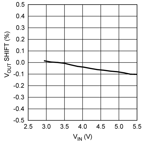
Line Regulation
