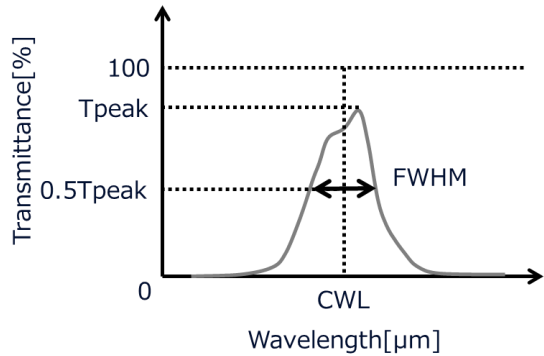
Figure 10.1 Definition of CWL, FWHM and Tpeak
