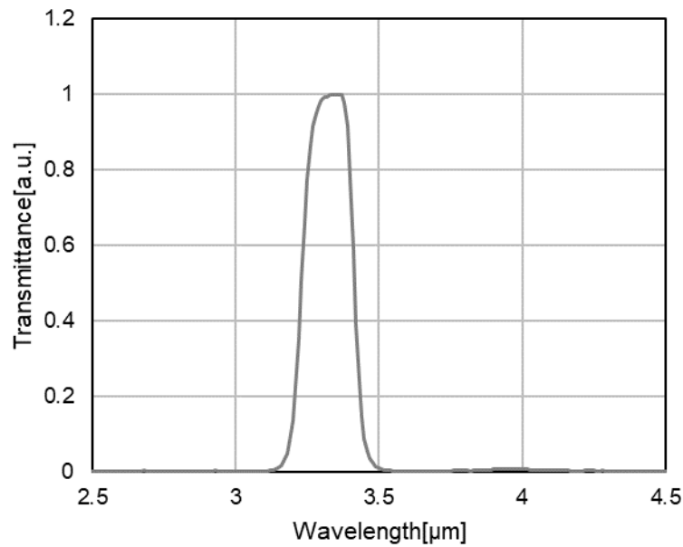
Figure 10.2 Optical filter transmittance (Reference)
