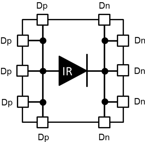
Figure 5.1 Block Diagram
