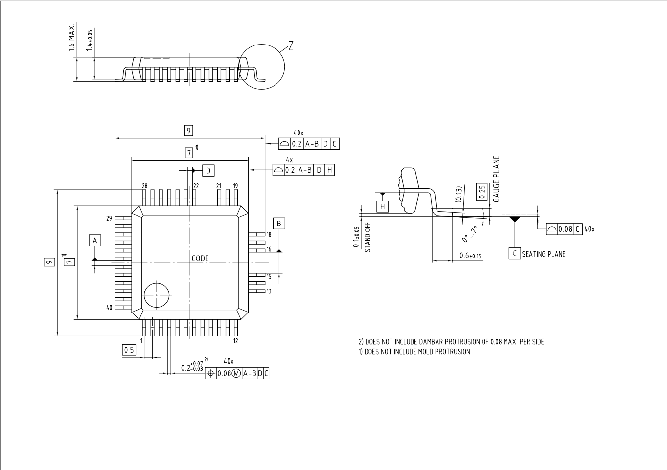
Figure 20 PG-LQFP-40-1
