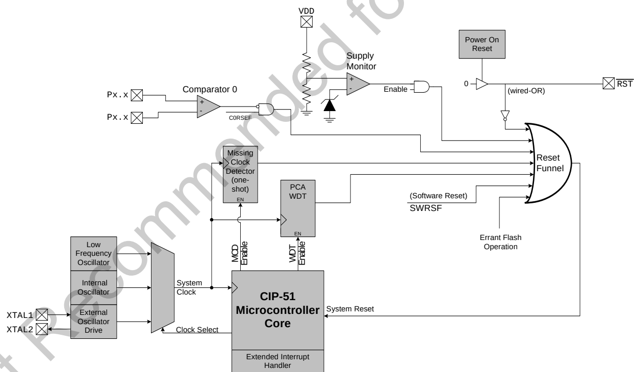
Figure 17.1. Reset Sources
