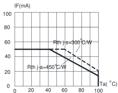
FIG.5 RED&amp;AMBER MAXIMUM FORWARD DC CURRENT VS AMBIENT TEMPERATURE (Tjmax=110 °C)
