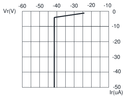
FIG.3 RED&amp;AMBER REVERSE CURRENT VS. REVERSE VOLTAGE.
