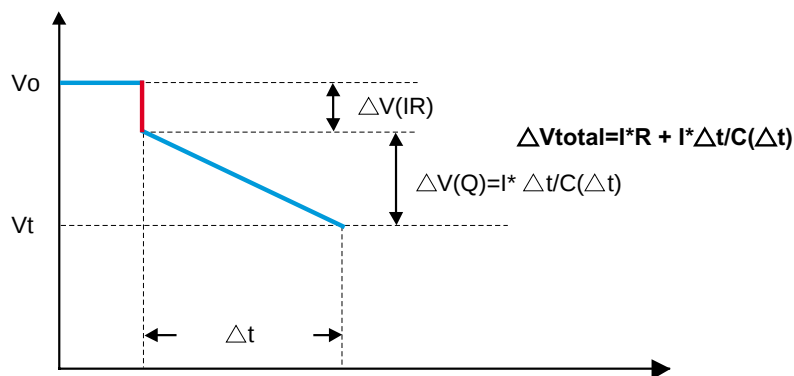
Fig 4 Voltage-time relation of capacitor unit
