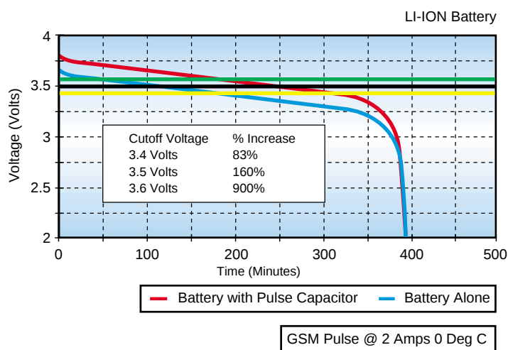
Fig. 6b Battery Life at 0°C
