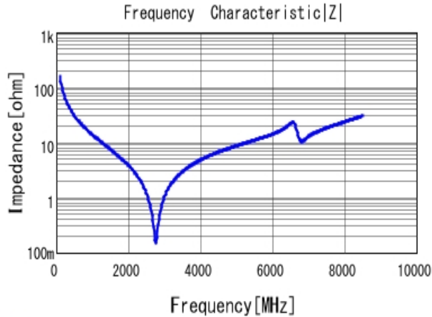
■ GJM1551C1H100FB01 |Z| DC0V, 20degC
