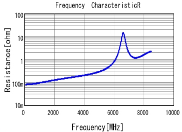
■ GJM1551C1H100FB01 R DC0V, 20degC
