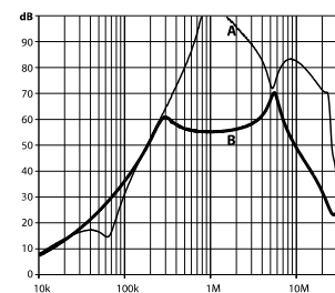
20 A types
