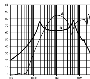
8 A types
