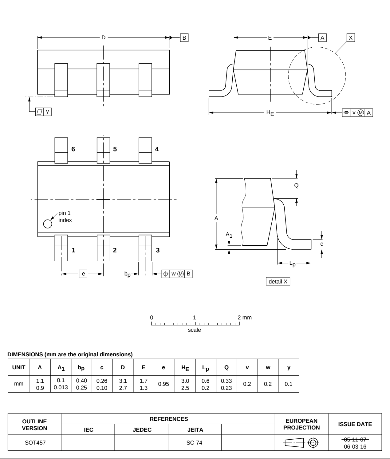
Fig 11. SOT457 (TSOP6)
