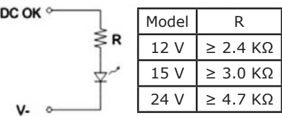
(b)LED
