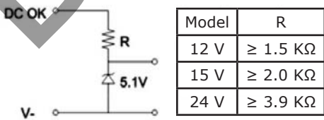
(a)5V signal
