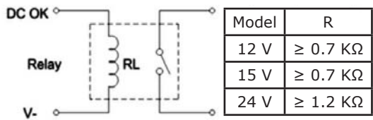
(c)Relay
