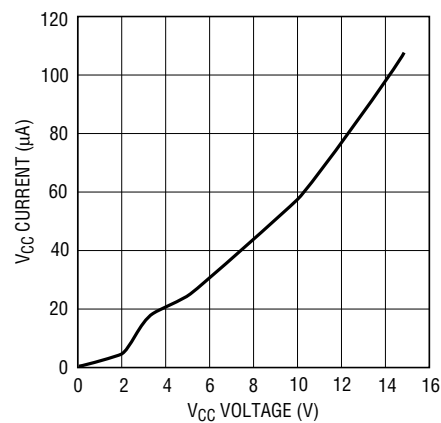
V_{CC} Shutdown Current vs V_{CC} Voltage
