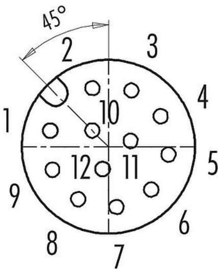
Contact arrangement (Plug-in side)
