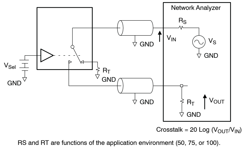
Figure 10. Non-Adjacent Channel-to-Channel Crosstalk
