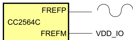
Figure 6-4. Clock Configuration (Sine Wave, DC-Coupled)
