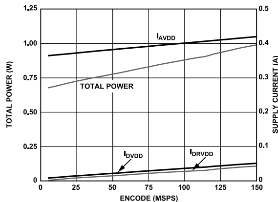
Figure 63. AD9600-150 Power and Current vs. Sample Rate
