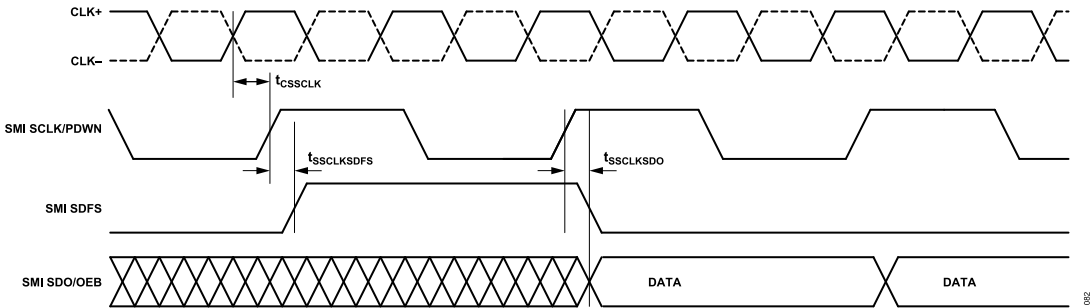
Figure 5. Signal Monitor SPORT Output Timing (Divide-by-2 Mode)
