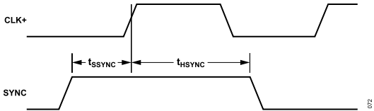
Figure 4. SYNC Input Timing Requirements
