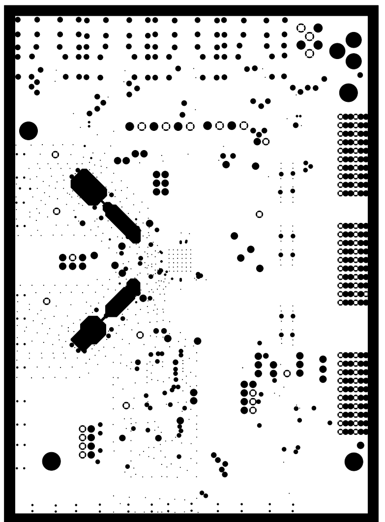
Figure 88. Evaluation Board Layout, Ground Plane
