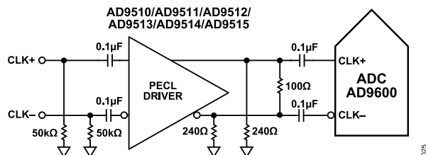
Figure 58. Differential PECL Sample Clock (up to 150 MSPS)
