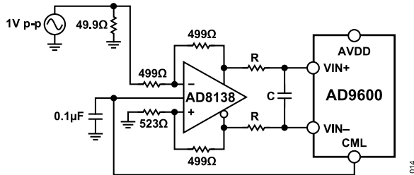
Figure 46. Differential Input Configuration Using the AD8138
