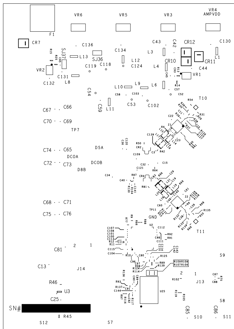
Figure 91. Evaluation Board Layout, Silk Screen, Secondary Side
