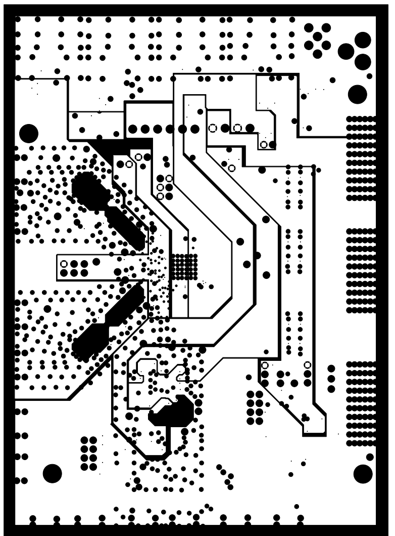
Figure 87. Evaluation Board Layout, Power Plane
