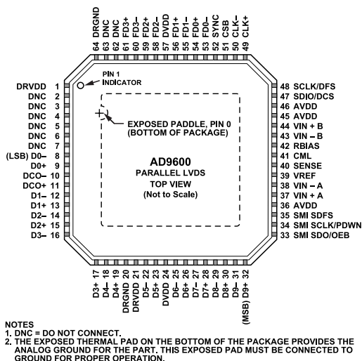
Figure 7. Interleaved Parallel LVDS Mode Pin Configuration (Top View)
