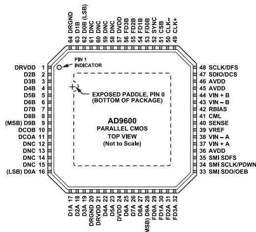
Figure 6. Parallel CMOS Mode Pin Configuration (Top View)
