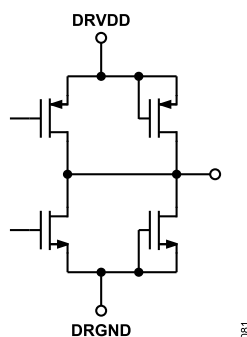
Figure 10. Digital Output
