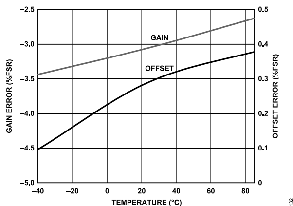
Figure 32. AD9600-150 Gain and Offset vs. Temperature
