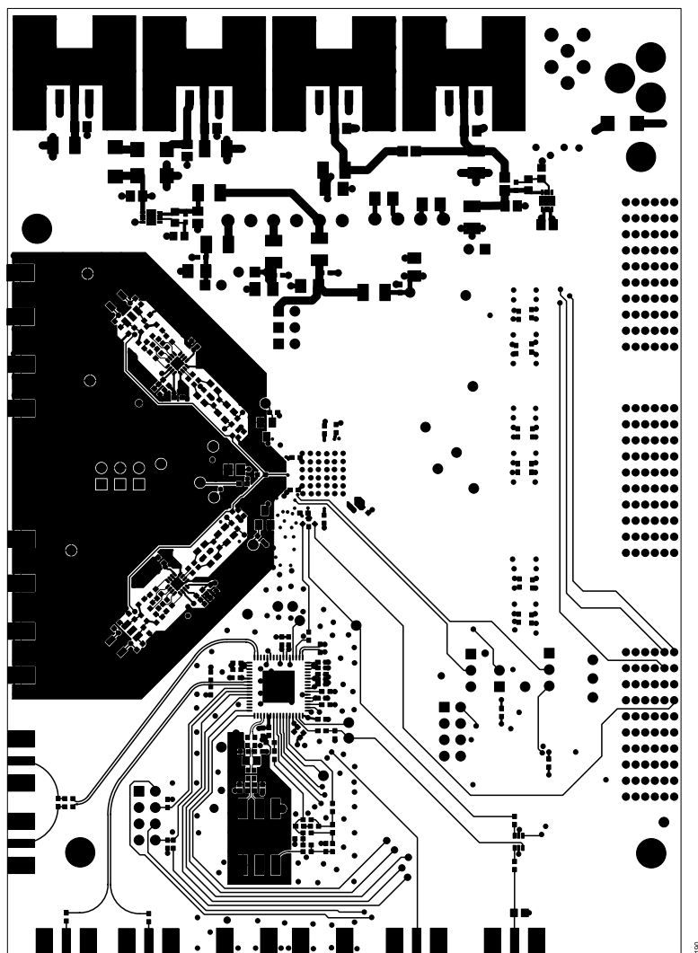
Figure 89. Evaluation Board Layout, Secondary Side (Mirrored Image)
