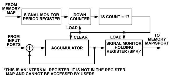
Figure 68. ADC Input RMS Magnitude Monitoring Block Diagram
