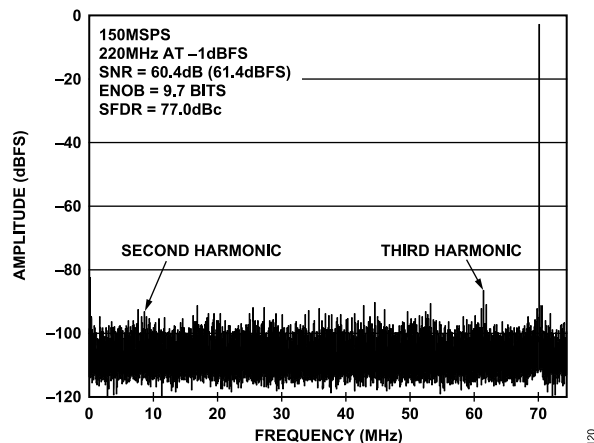
Figure 20. AD9600-150 Single-Tone FFT with f_{IN} = 220\text{ MHz}
