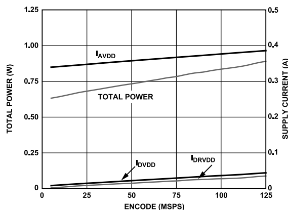
Figure 64. AD9600-125 Power and Current vs. Sample Rate
