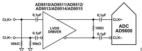
Figure 59. Differential LVDS Sample Clock (up to 150 MSPS)
