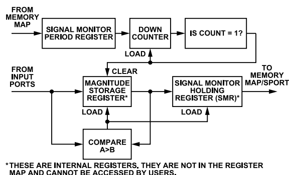
Figure 67. ADC Input Peak Detector Block Diagram
