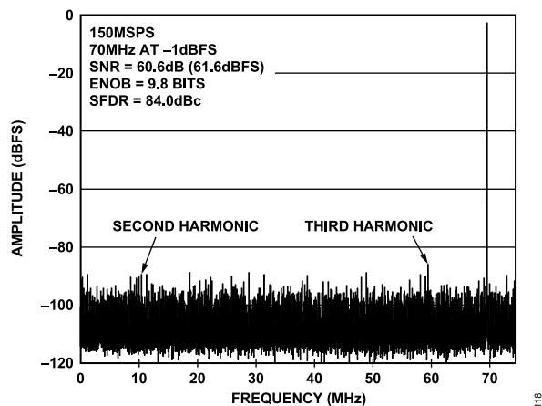
Figure 18. AD9600-150 Single-Tone FFT with f_{IN} = 70\text{ MHz}
