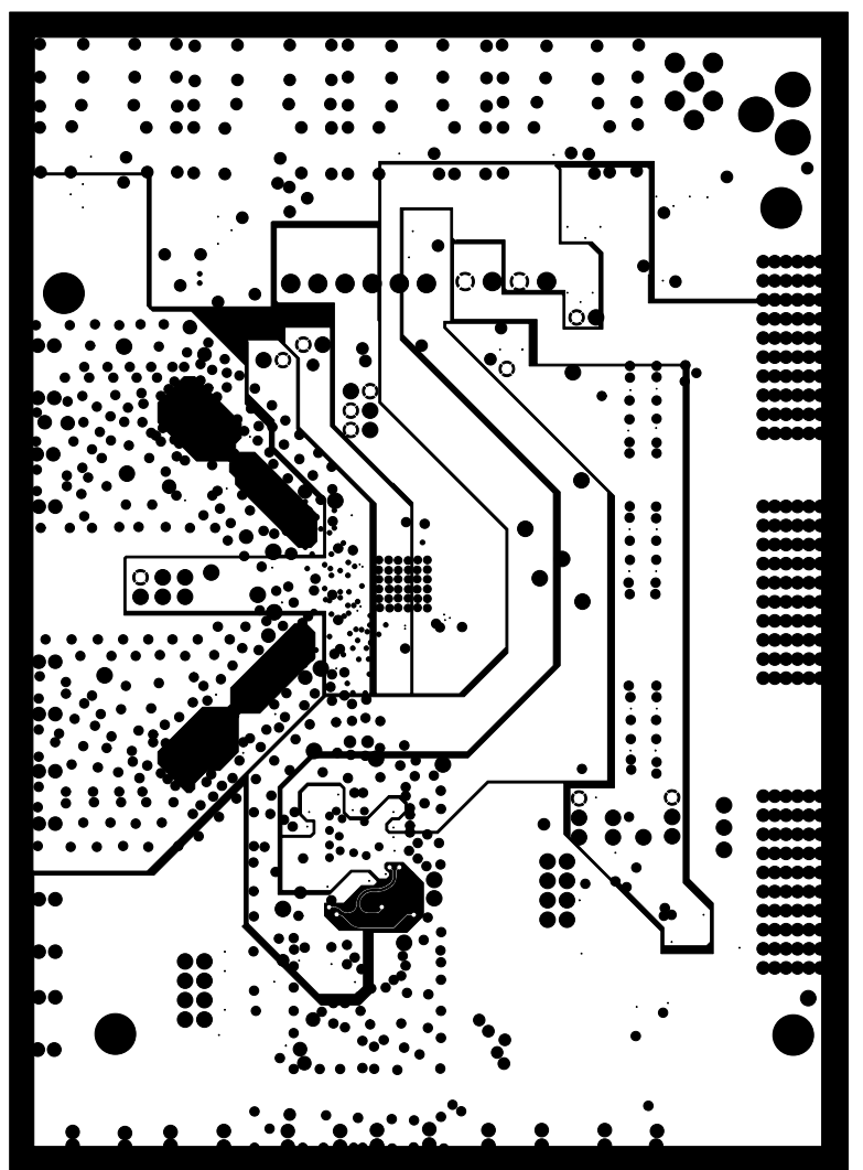
Figure 86. Evaluation Board Layout, Power Plane
