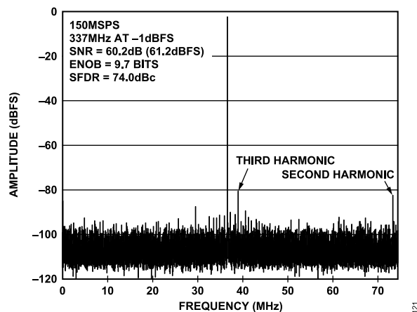
Figure 21. AD9600-150 Single-Tone FFT with f_{IN} = 337\text{ MHz}
