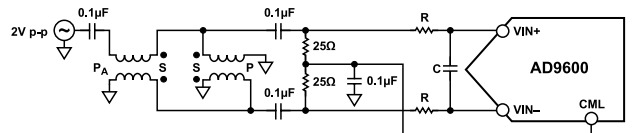
Figure 49. Differential Double-Balun Input Configuration
