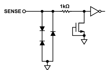
Figure 13. Equivalent SENSE Circuit
