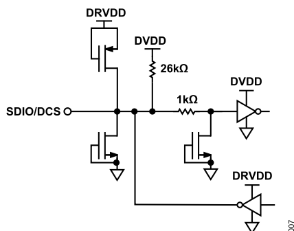
Figure 11. Equivalent SDIO/DCS Input Circuit
