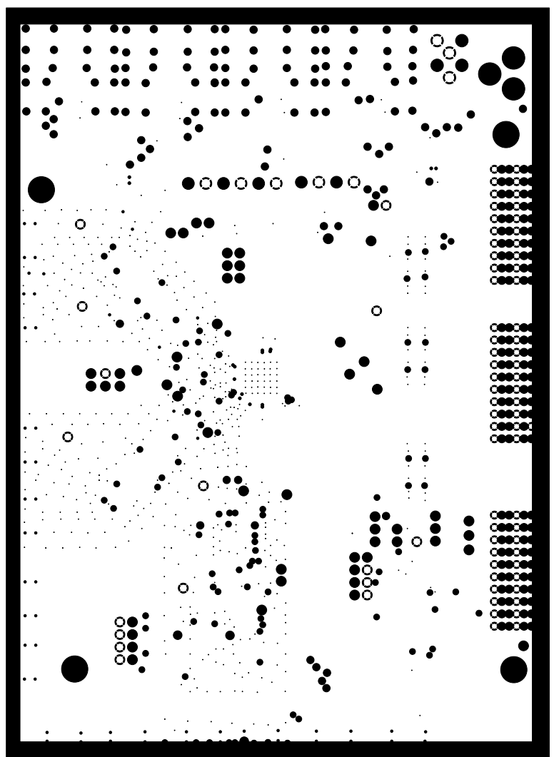
Figure 85. Evaluation Board Layout, Ground Plane
