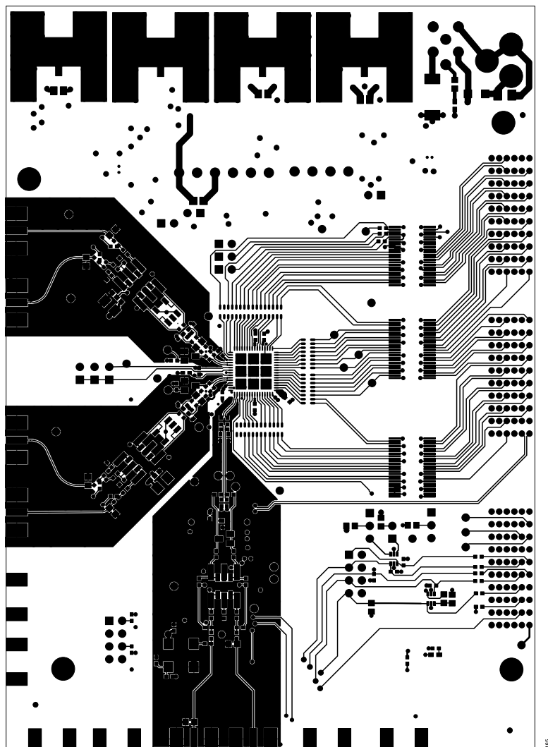
Figure 84. Evaluation Board Layout, Primary Side
