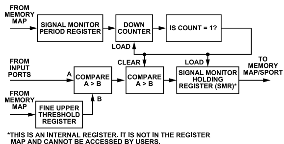
Figure 69. ADC Input Threshold Crossing Block Diagram
