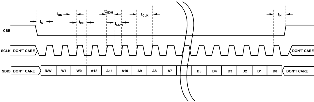
Figure 72. Serial Port Interface Timing Diagram
