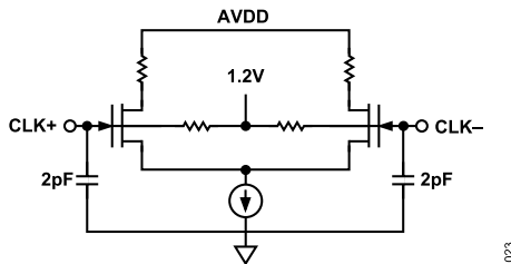
Figure 55. Equivalent Clock Input Circuit
