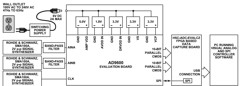
Figure 73. Evaluation Board Connection
