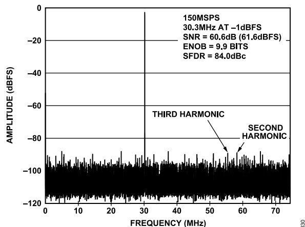
Figure 17. AD9600-150 Single-Tone FFT with f_{IN} = 30.3\text{ MHz}
