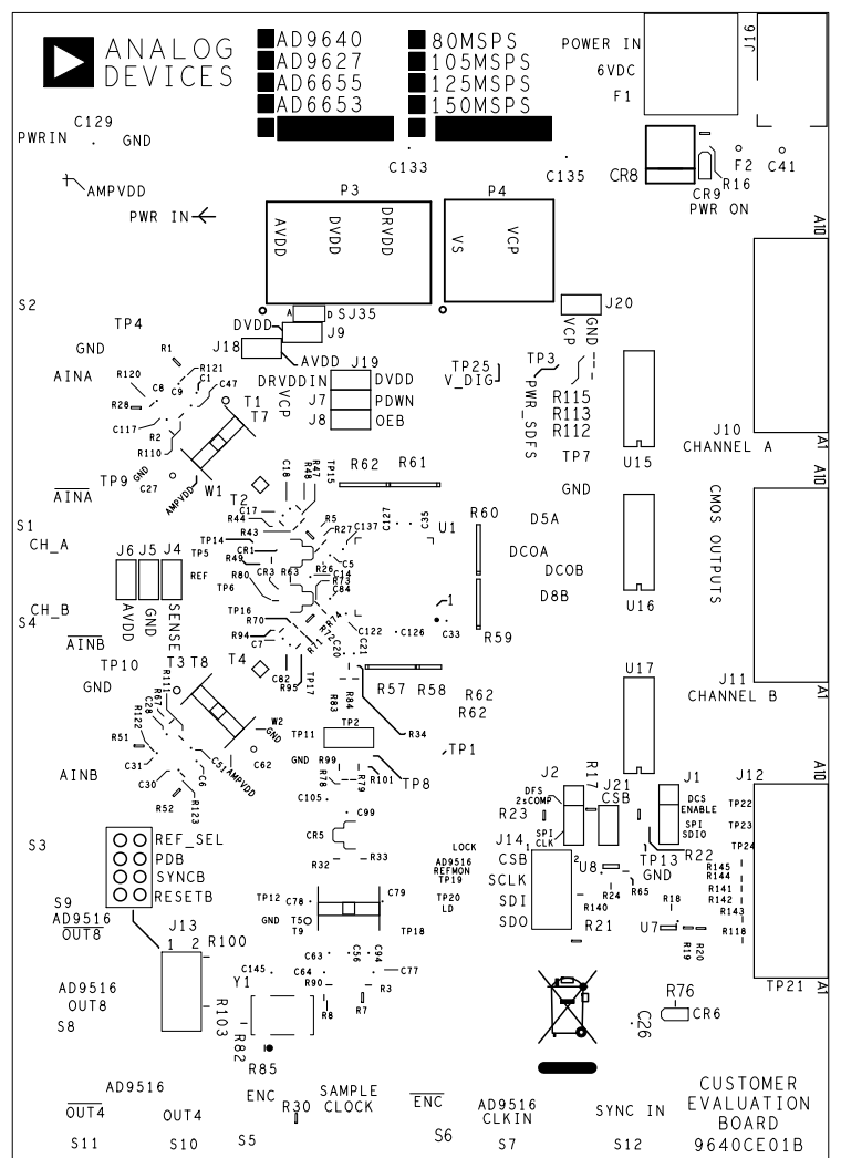
Figure 90. Evaluation Board Layout, Silkscreen, Primary Side
