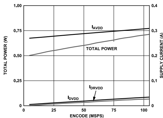
Figure 65. AD9600-105 Power and Current vs. Sample Rate
