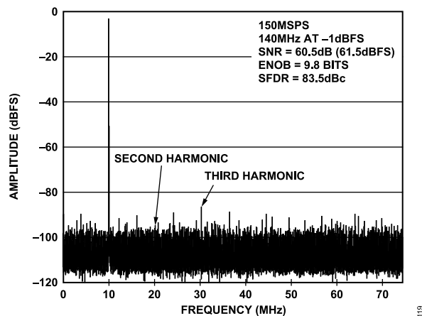
Figure 19. AD9600-150 Single-Tone FFT with f_{IN} = 140\text{ MHz}
