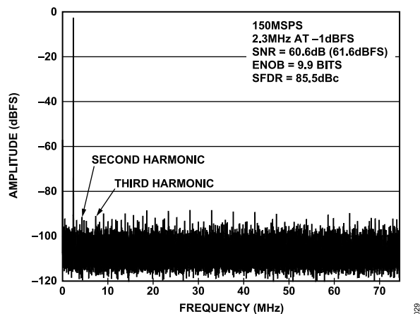
Figure 16. AD9600-150 Single-Tone FFT with f_{IN} = 2.3\text{ MHz}
