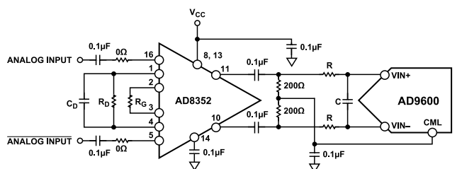
Figure 50. Differential Input Configuration Using the AD8352
