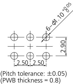
PWB mounting hole for reference
