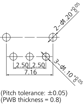
PWB mounting hole for reference
