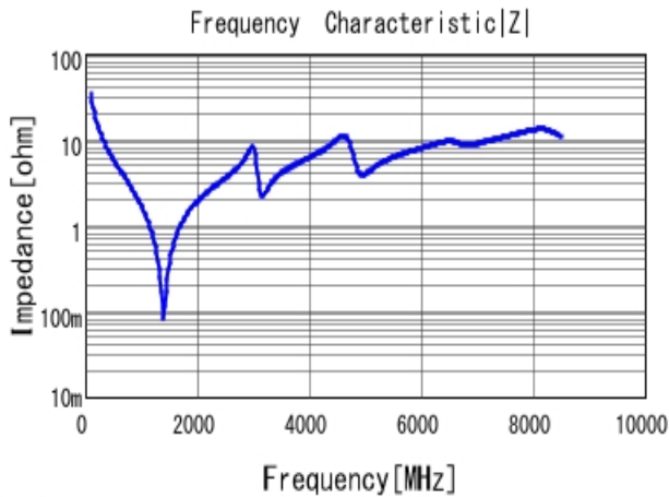
■ GQM1555C2A470GB01 |Z| DC0V, 25degC
