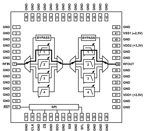
Figure 30. ADMV8818-EP Configured for HPF 1 and LPF 1
