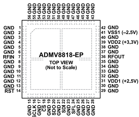
Figure 3. Pin Configuration
