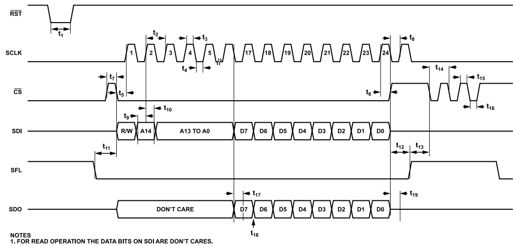
Figure 2. Timing Diagram
