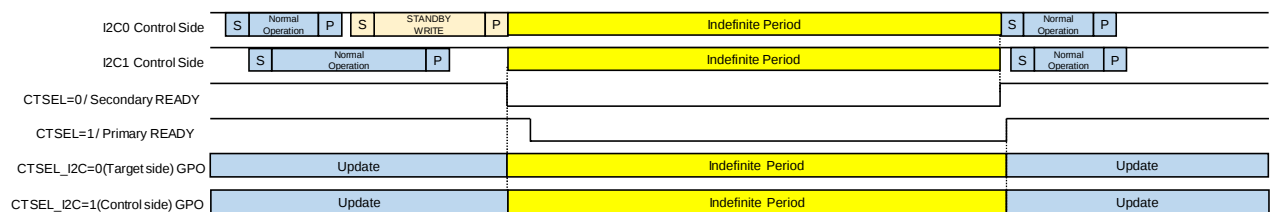
Figure 28 Normal => Standby (CTSEL_I2C=0/Secondary , CTSEL_I2C=1/Primary)
