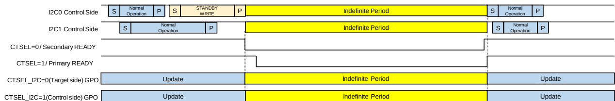
Figure 30 Standby => Normal (CTSEL_I2C=0/Secondary, CTSEL_I2C=1/Primary)
