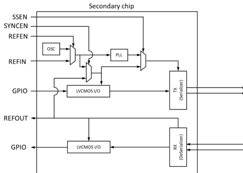
Figure 3 Clock Tree diagram of Secondary chip
