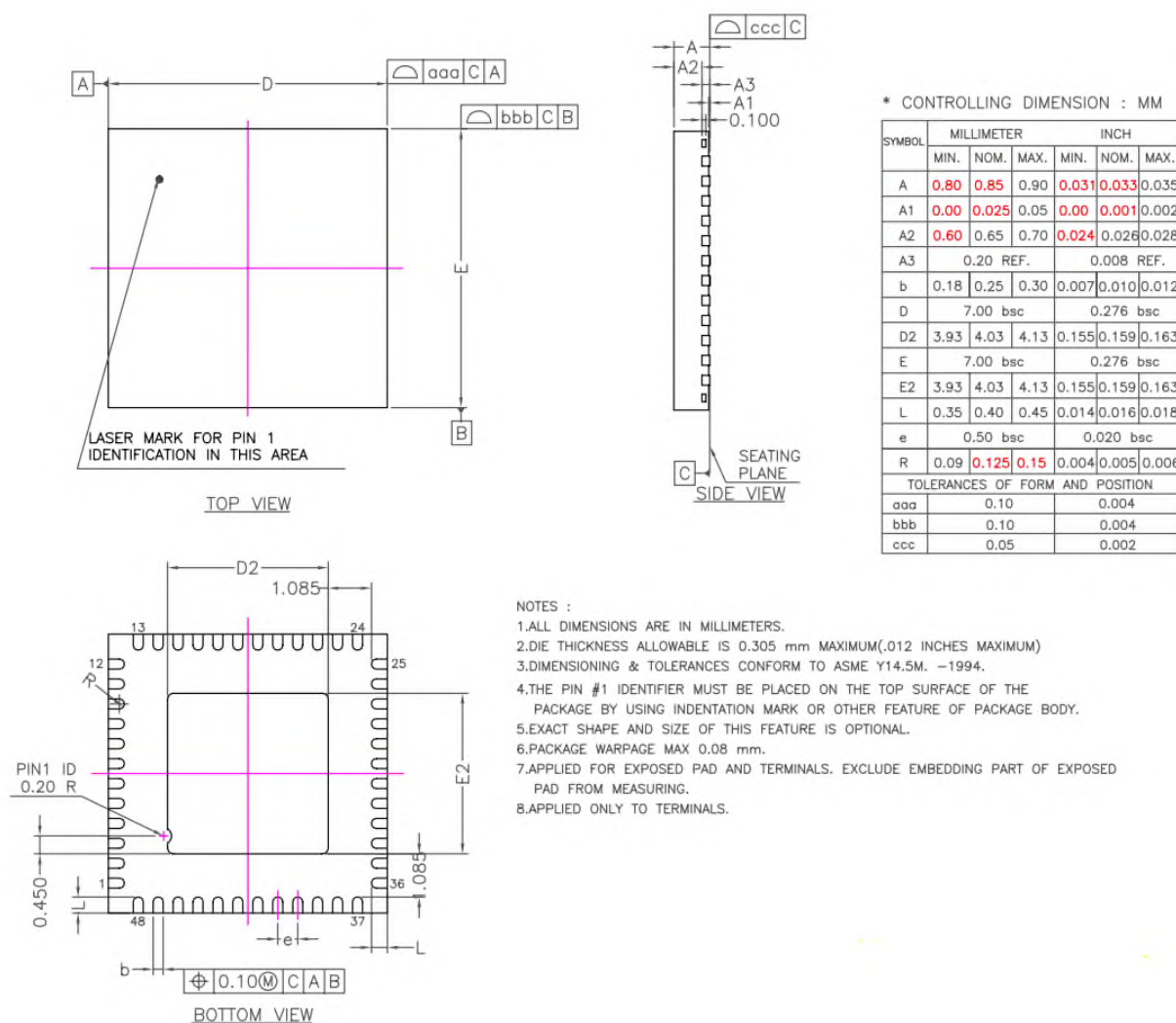
Figure 31 48-pin QFN package physical dimension
