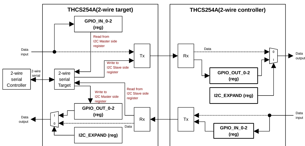
Figure 22 2-wire serial expander function
