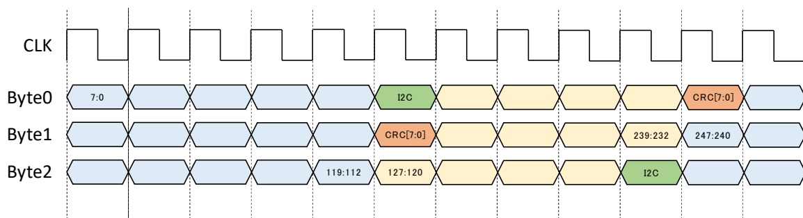
Figure 26 CRC data
