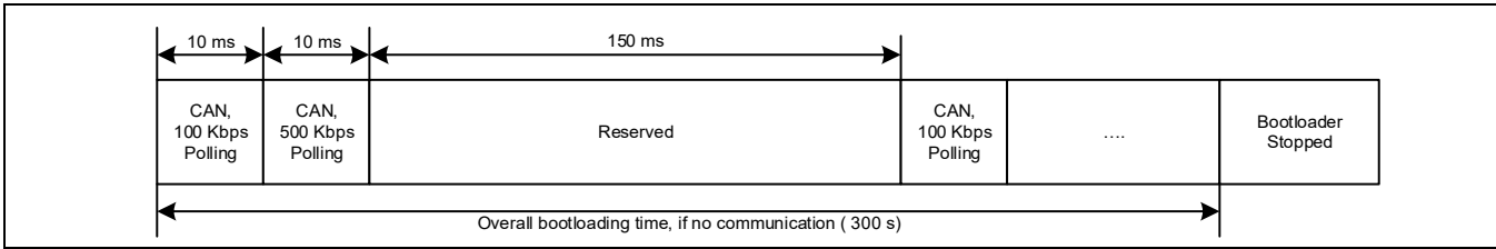
Figure 29-1 Bootloading sequence
