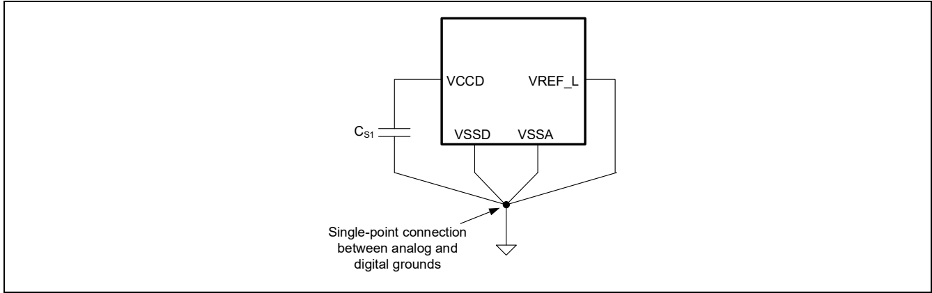
Figure 26-2 Smoothing capacitor
