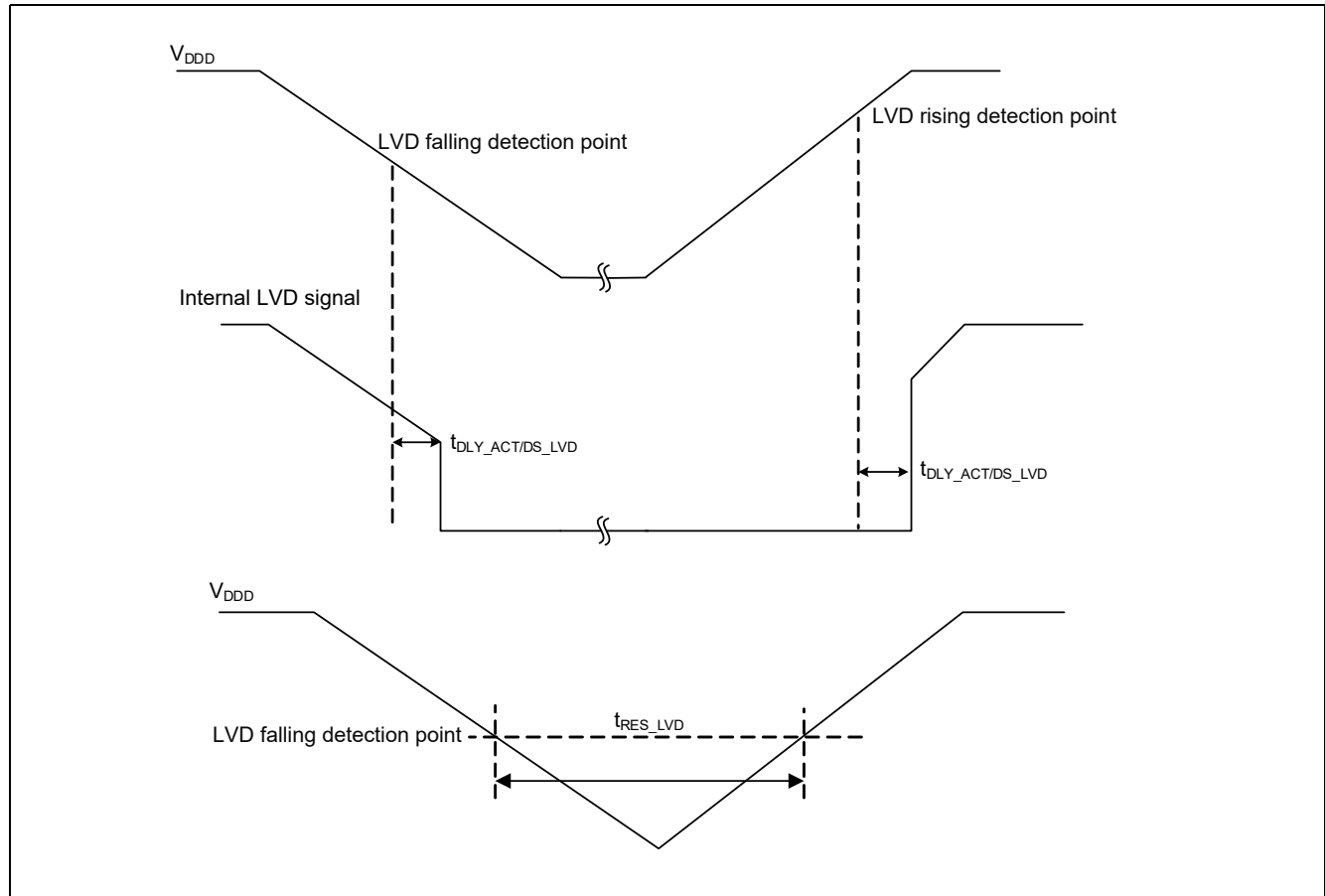
Figure 26-20 LVD specifications
