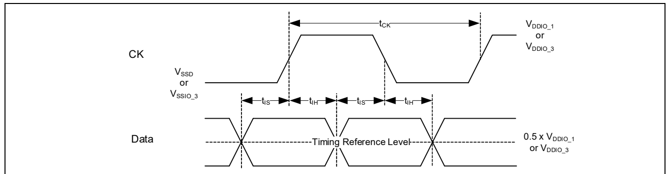
Figure 26-46 HYPERBUS™ timing reference level
