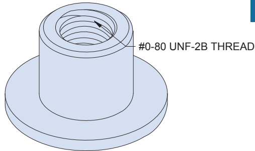
PCB Mount Fasteners
