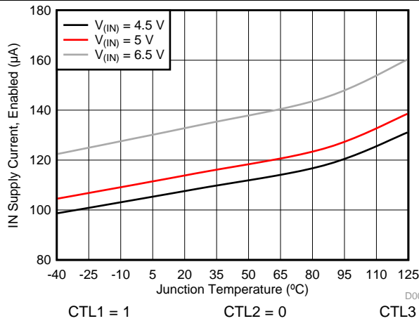
Figure 9. Enabled IN Supply Current – Client Mode (100) vs Temperature
