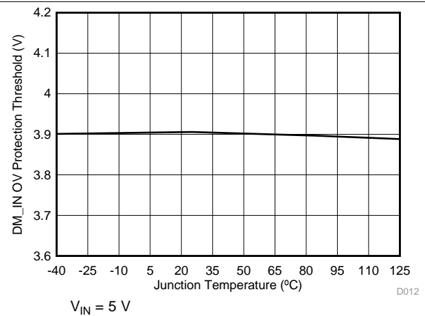
Figure 12. DM_IN Overvoltage Protection Threshold vs Temperature
