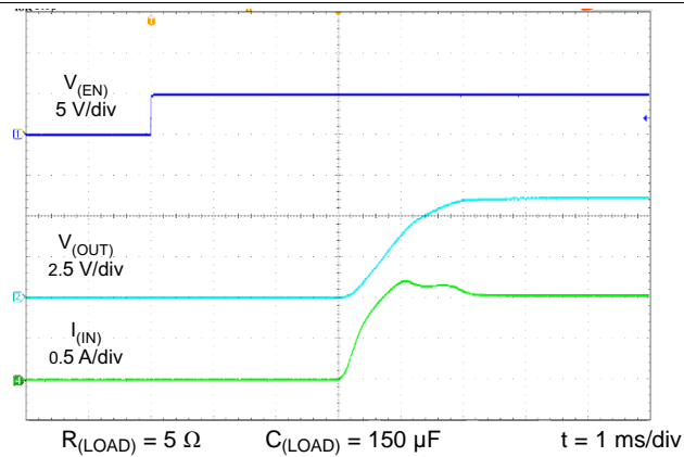
Figure 20. Turnon Response
