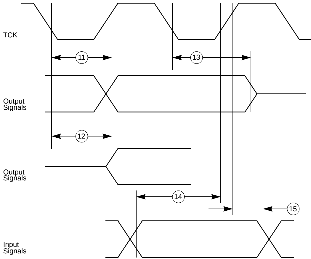
Figure 24. JTAG boundary scan timing
