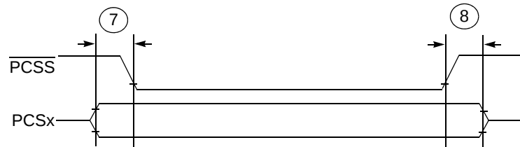
Figure 38. DSPI PCS strobe ( \overline{\text{PCSS}} ) timing
