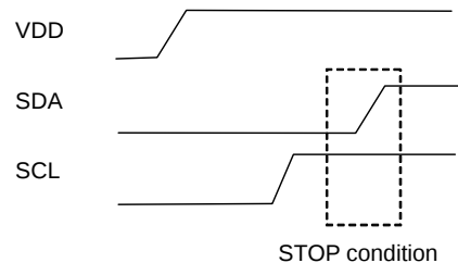
Figure 21. STOP Condition
