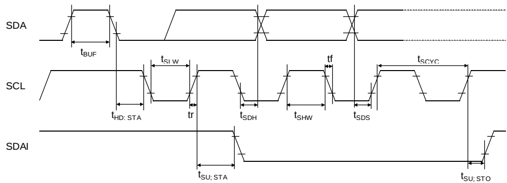
Figure 5. Interface Timing
