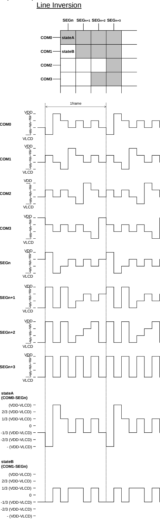
Figure 14. LCD Waveform at Line Inversion (1/3bias)
