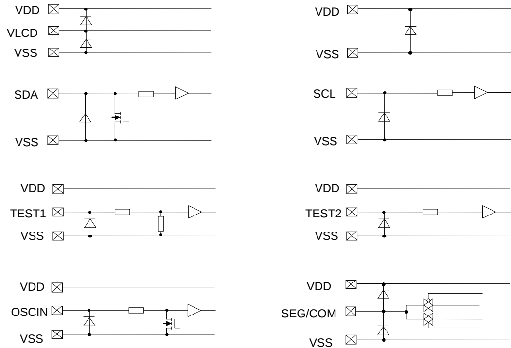
Figure 6. I/O Equivalence Circuit
