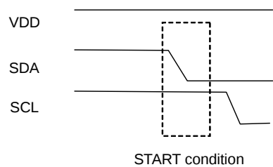
Figure 22. START Condition
