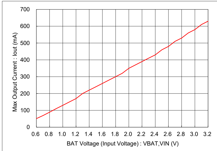
(4) Max Output Current vs BAT Voltage(Input Voltage) @ Ta=25°C
