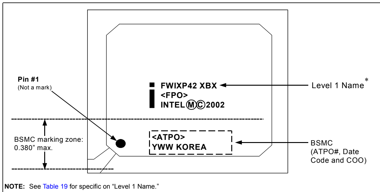
Figure 7. Package Markings
