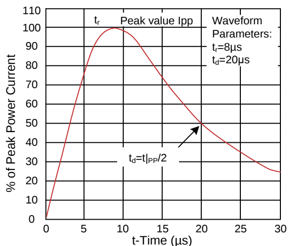
Figure 2. Pulse Waveform
