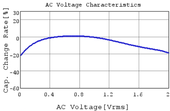
GRM188R60J476ME01 C-AC Voltage capchange, D
