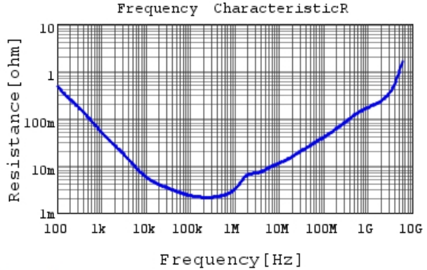
GRM188R60J476ME01 R DCOV,25degC
