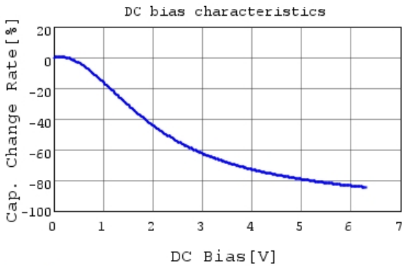
GRM188R60J476ME01 C-DC bias capchange, 25.0C
