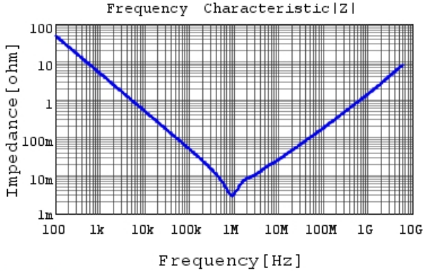
GRM188R60J476ME01 |Z| DCOV,25degC
