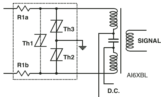
Figure 16. ISDN Protection
