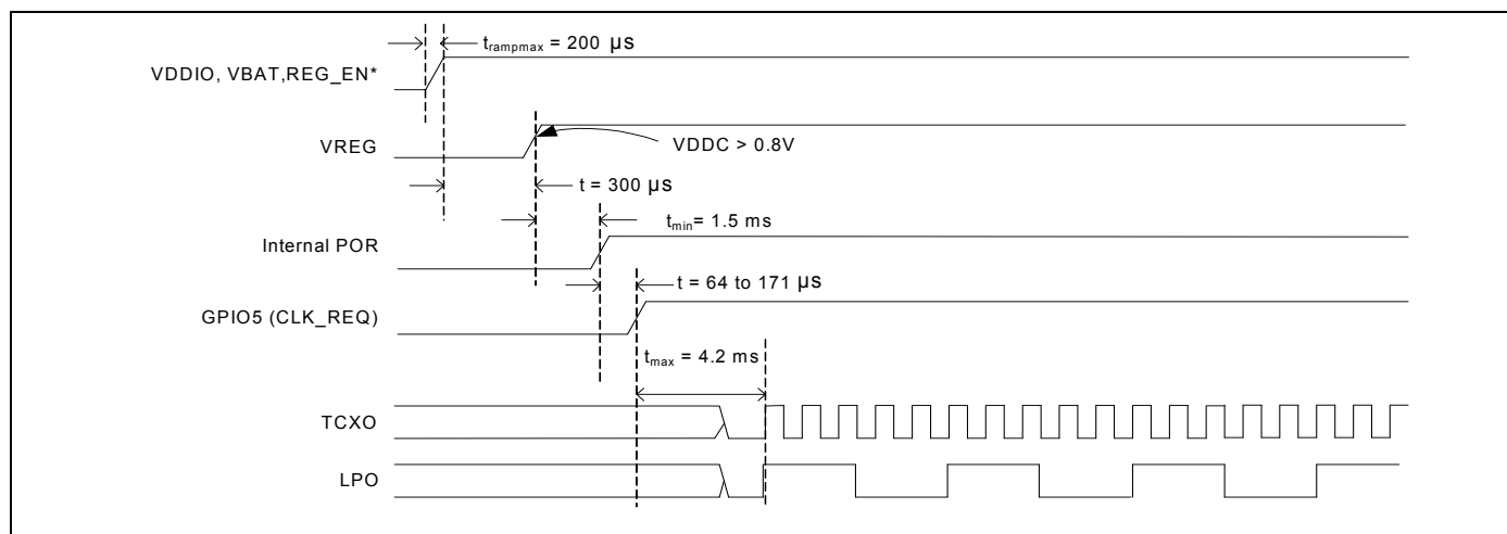
Figure 11. Startup Timing from Power-on Reset
