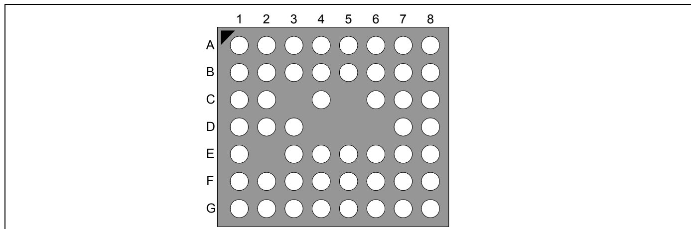
Figure 8. 50-Ball 4.5 x 4 x 0.6 mm (FPBGA) Array
