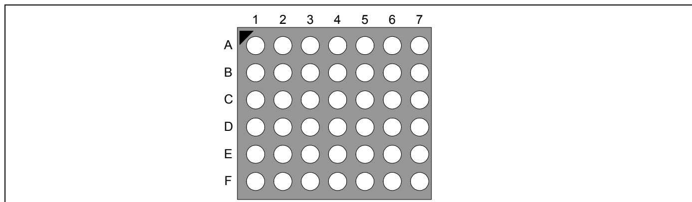
Figure 9. 42-Bump 2.97 x 2.46 x 0.5 mm Array (Top View)
