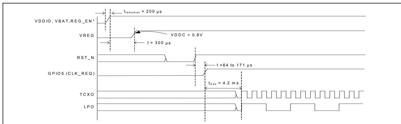
Figure 10. Startup Timing from RST_N
